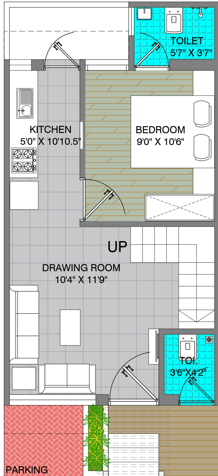
GROUND FLOOR CONSTRUCTION AREA 40.85 SQ.MT
