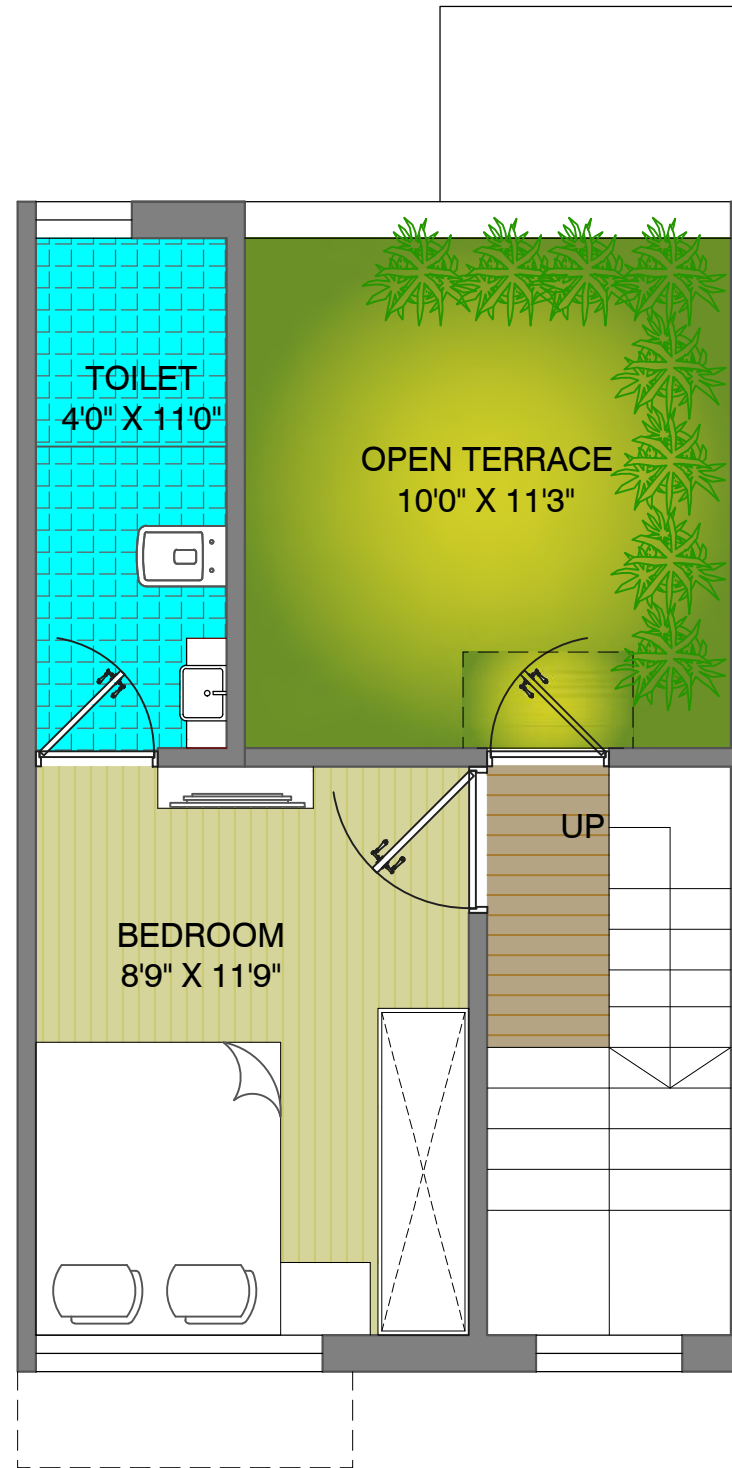
FIRST FLOOR CONSTRUCTION AREA 24.55 SQ.MT
