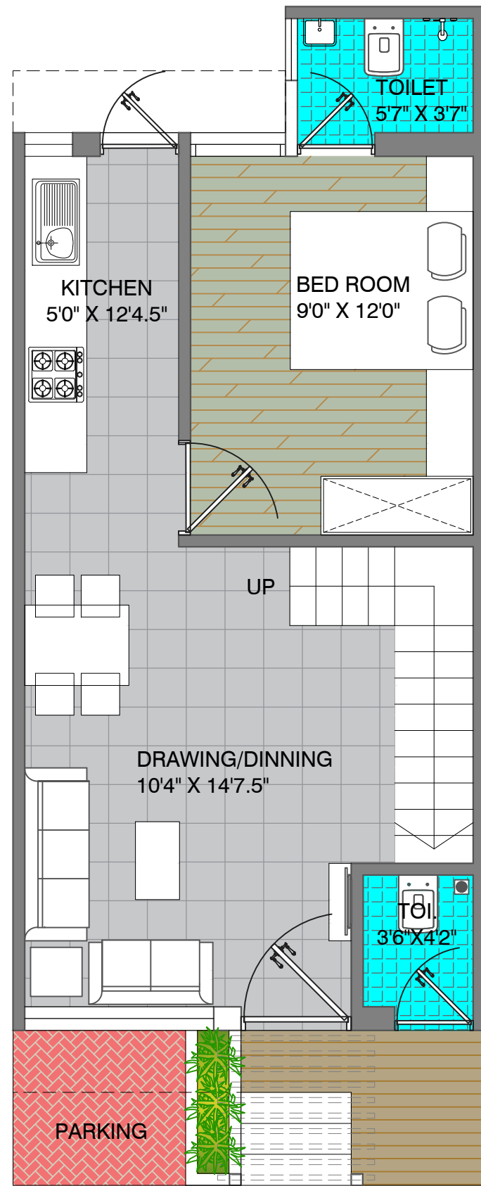
GROUND FLOOR CONSTRUCTION AREA 47.15 SQ.MT
