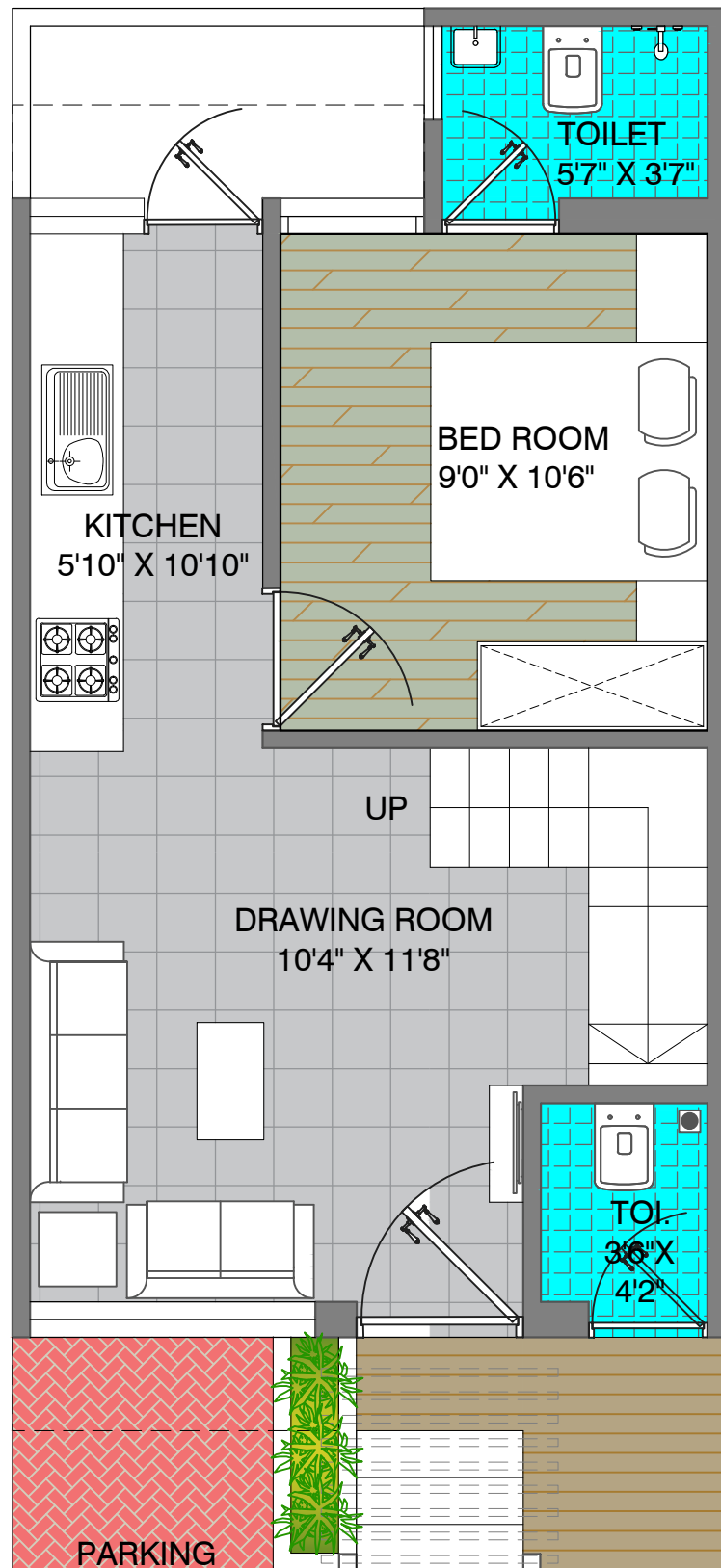
GROUND FLOOR CONSTRUCTION AREA 40.84 SQ.MT
